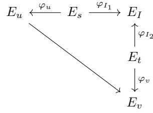
FIGURE 2. The isogenies in the algorithm IdealTolsogeny .
